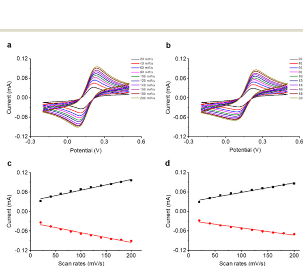
Fig. 2 Cyclic voltammetric curves of (a) Aptasensor 1 and (b) Aptasensor 2 as a function of potential (–0.2–0.6 V). Plotting the current intensity of (c) Aptasensor 1 and (d) Aptasensor 2 with different scan rates (20–200 mV s -1 ).
