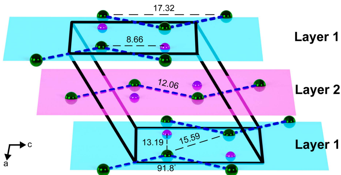
Fig. 2 Simplified unit cell depiction of \{[\text{Cp}_2^*\text{Dy}(\text{bpy})][\text{BPh}_4]\}_n , 3, in a crystal of \{[\text{Cp}_2^*\text{Dy}(\text{bpy})][\text{BPh}_4] \cdot 3(\text{C}_4\text{H}_8\text{O})\}_n along the ac plane illustrating the organisation of the layers with respect to each other. Green and purple spheres represent Dy and B atoms (where B is the boron atom of the (\text{BPh}_4)^- counteranion), respectively. The dashed blue lines represent the bridging bipyridyl ligands. N, C, and H atoms, as well as solvent molecules in the crystal lattice have been omitted for clarity. Distances and angles are given in Å and deg.
