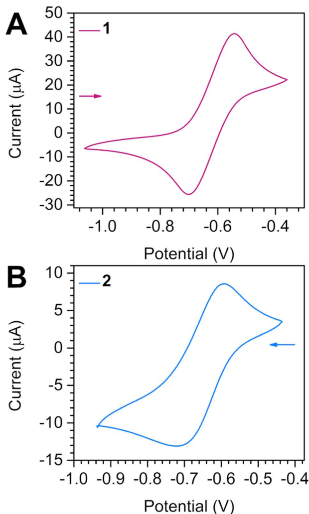
Fig. 3 Cyclic voltammograms of [(\text{Cp}^*_2\text{Dy})_2(\mu\text{-tan})] (1) (A) and [(\text{Cp}^*_2\text{Dy})_2(\mu\text{-tan}')] [\text{BARF}_{20}] (2) (B), measured in DCM at 300 K with 0.22 \text{ mmol L}^{-1} [\text{t}^+\text{Bu}_4\text{N}][\text{PF}_6] supporting electrolyte and 3 \text{ mmol L}^{-1} analyte concentration against a Ag wire pseudo reference electrode with a 100 \text{ mV s}^{-1} scan rate.
