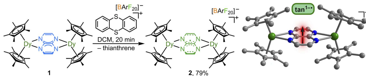
Fig. 4 Synthesis of [(\text{Cp}^*_2\text{Dy})_2(\mu\text{-tan}')] [\text{BARF}_{20}] (2) through oxidation of [(\text{Cp}^*_2\text{Dy})_2(\mu\text{-tan})] (1) with [\text{Thian}'] [\text{BARF}_{20}] (left). Structure of 2, obtained through single-crystal X-ray diffraction analysis (right). Green, blue, and grey spheres represent dysprosium, nitrogen, and carbon atoms, respectively. All hydrogen atoms and the counter ion [\text{BARF}_{20}]^- are omitted for clarity.
