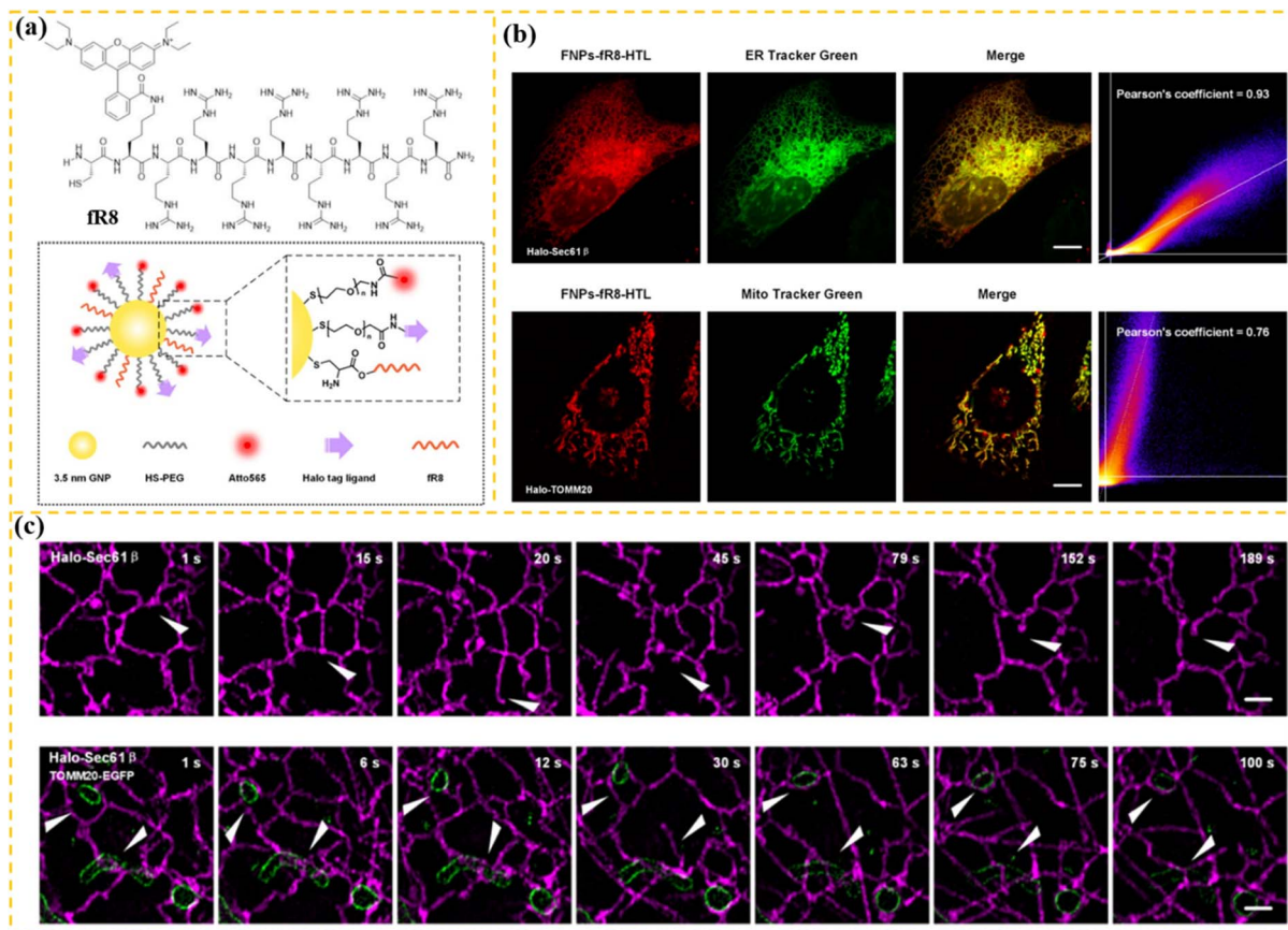
Fig. 59 (a) Chemical structure of the peptide sequence fR8 and design process of nanoprobe FNP-fR8-HTL. (b) Co localization imaging of probe FNP-fR8-HTL in U-2OS cells. (c) Delayed SIM imaging of probe FNP-fR8-HTL in U-2OS cells and SIM imaging of mitochondrial endoplasmic reticulum interaction. Reprinted with permission from American Chemical Society, copyright 2024, as cited in ref. 138.
