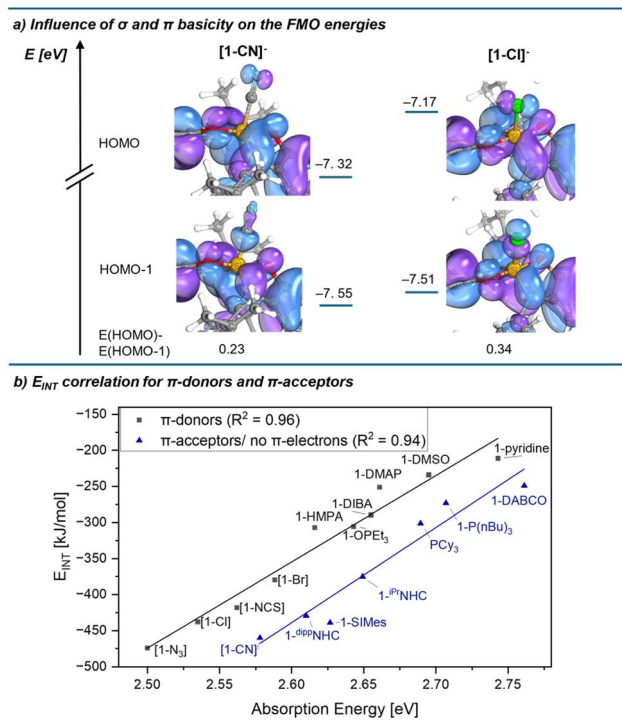
Fig. 9 (a) Influence of \pi -basicity on the energy of occupied molecular orbitals ( 1 -CN − vs. 1 -Cl − ). (b) Correlation of the absorption energy of donor adducts (excluding outliers) with the interaction energy E_{\text{INT}} ( E - E_{\text{DEF}} , DSD-BLYP(D3BJ)/def2-TZVPP// r^2 SCAN-3c).
