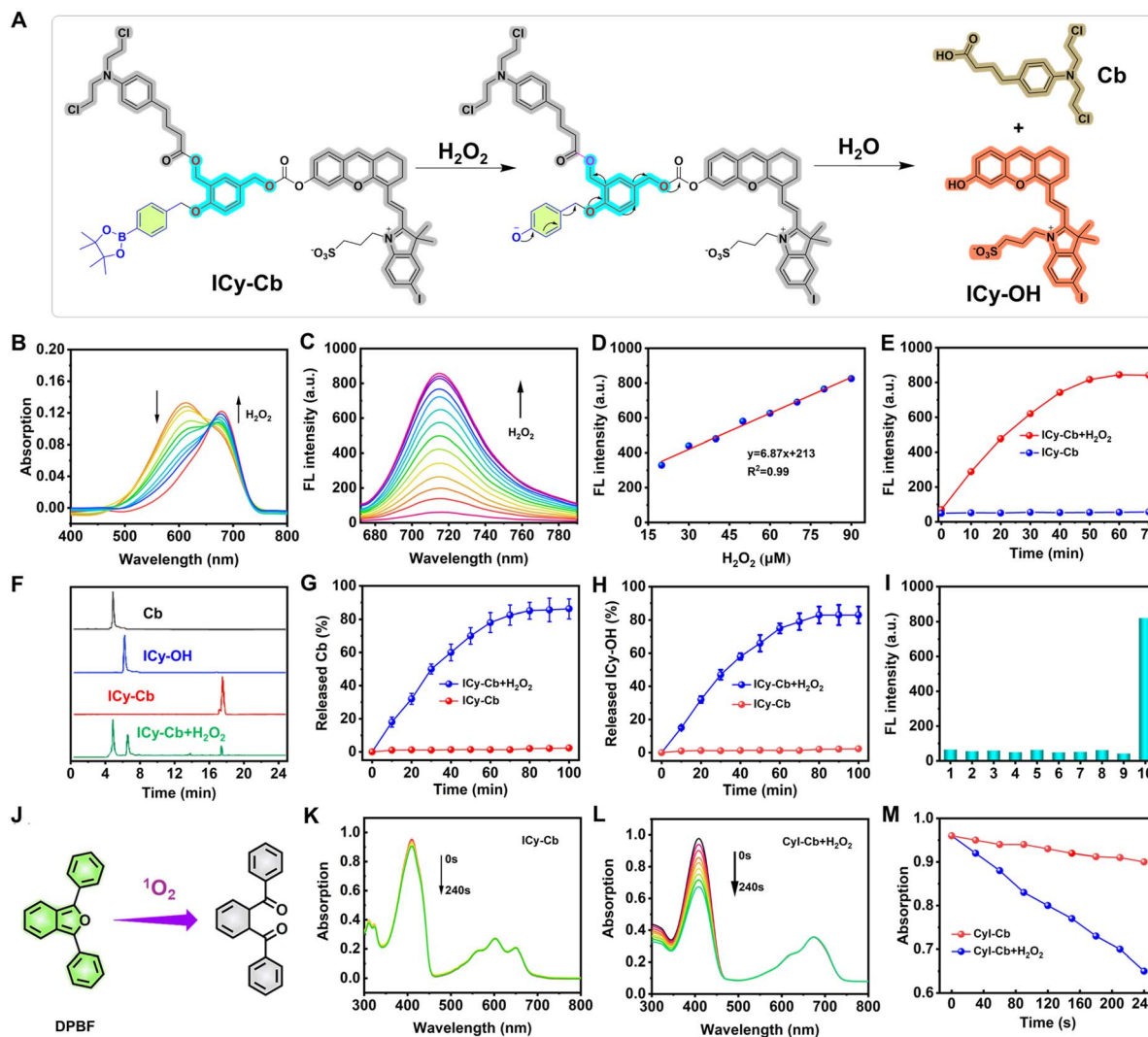
Fig. 1 (A) Schematic illustration of H 2 O 2 -mediated fluorescence turn-on and drug release of ICy-Cb. (B) UV-vis and (C) Fluorescence spectra absorbance changes of ICy-Cb (5 μM) in PBS buffer (10.0 mM, pH 7.4, containing 30% DMSO), after introduction of H 2 O 2 (0.0–100.0 μM). (D) The linear relationship between I 720 nm and the concentration of H 2 O 2 (20.0–90.0 μM). (E) Time-dependent fluorescence of ICy-Cb with the addition of H 2 O 2 (100.0 μM) in PBS buffer (10.0 mM, pH 7.4, containing 30% DMSO). (F) HPLC chromatographic analysis was performed on several samples: pure Cb (black), ICy-OH (blue), ICy-Cb (red), and a mixture (green) of ICy-Cb and H 2 O 2 . Release efficiency of (G) Cb and (H) ICy-OH from ICy-Cb. (I) Fluorescence measurements of ICy-Cb (5.0 μM) were recorded in response to H 2 O 2 (100.0 μM) and various other substances (100.0 μM): (1) Blank, (2) NO, (3) ONOO − , (4) • OH, (5) 1 O 2 , (6) O 2 •− , (7) ROO • , (8) t -BuO • , (9) HClO and (10) H 2 O 2 . All measurements were taken 90 minutes after adding the stimulants at room temperature, using an excitation wavelength of 670 nm and an emission wavelength of 720 nm. (J) Schematic illustration of DPBF detecting 1 O 2 . Photodegradation curves of DPBF in the presence of ICy-Cb (K) and ICy-Cb + H 2 O 2 (L) were obtained under 660 nm light irradiation for varying durations (0–240 s). (M) DPBF degradation (monitored at 415 nm) induced by ICy-Cb and ICy-OH under irradiation 660 nm.
