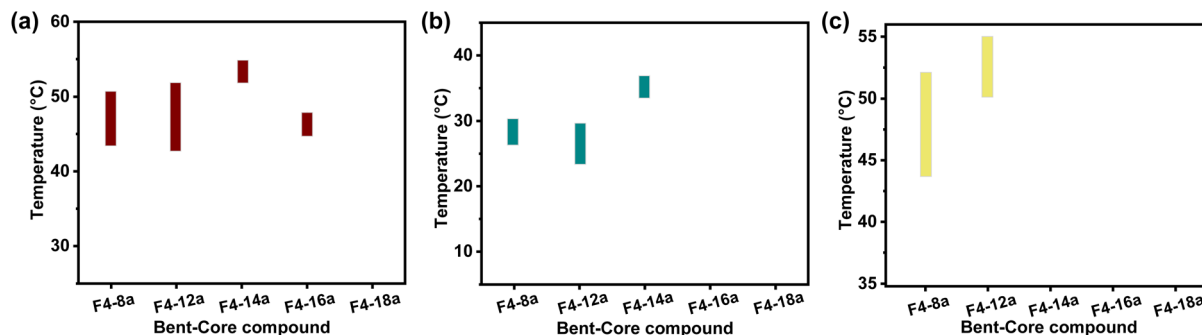
Fig. 11 Graphical representation illustrating the temperature range of BP formation as a function of varying homologues of F4-na series (a)–(c) correspond to compositions of 35 : 45 : 20, 25 : 45 : 30, and 45 : 25 : 30 weight percent of F4-na :5CB:S811, respectively.
