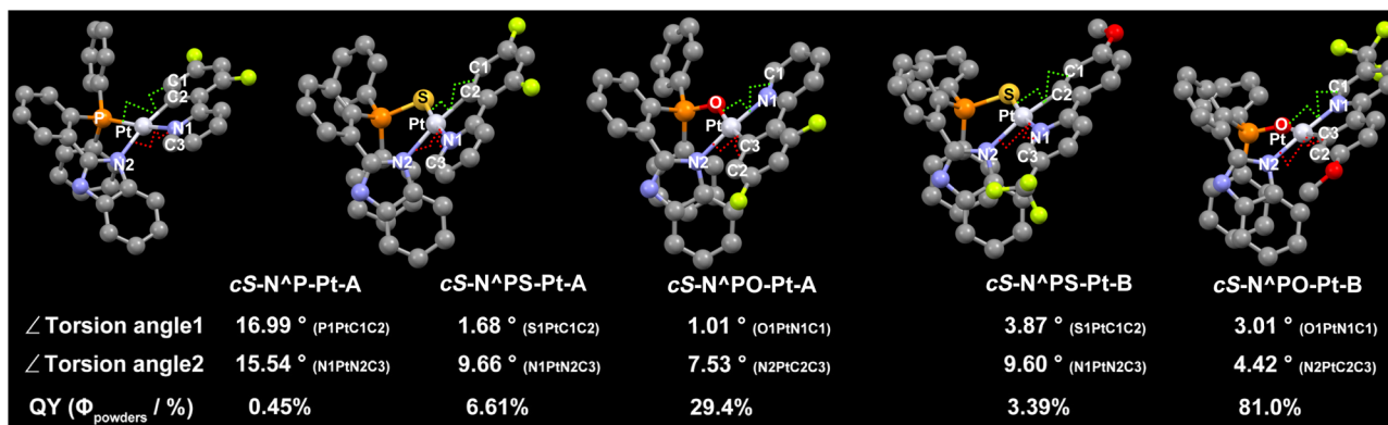
Fig. 7 The relationship between emission quantum yields and torsion angles of coordinated atoms among the representative products: cS-N A P-Pt-A, cS-N A PS-Pt-A, cS-N A PO-Pt-A, cS-N A PS-Pt-B, and cS-N A PO-Pt-B.
