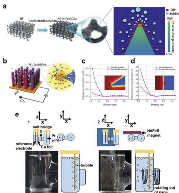
Fig. 7 (a) Schematic of Ni x Fe 1-x alloy nanocone synthesis and the formation of local electric field. Reproduced with permission from ref. 115 Copyright 2021 Wiley. (b) Schematic of wattle-like Pt-Ni to enhance mass transfer. (c and d) Simulations of hydrogen and potassium ion concentrations at the tip and the plane. Reproduced with permission from ref. 116 Copyright 2021 Royal Society of Chemistry. (e) Actual diagram of the action of magnetic fields on electrocatalytic CO 2 RR to improve the mass transfer. Reproduced with permission from ref. 117 Copyright 2021 Elsevier.
