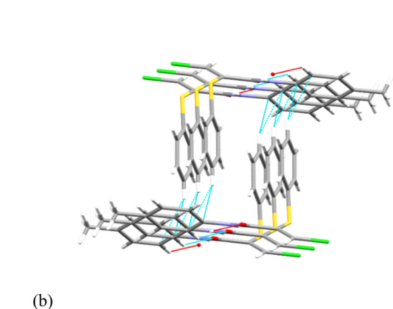
Fig. 5 Views, (a) and (b), from different angles showing the knitting of two chains of Z-3 together based on edge-to-face ( C-H\cdots\pi 2.83 Å) and face-to-face aromatic interactions.
