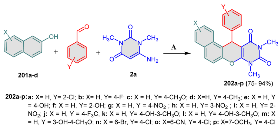
Scheme 75 Formation of chromeno[2,3-d]pyrimidines 202a–p. Reagents and conditions: A = \text{CHCl}_3 : \alpha -CAA (1 : 1), 90 °C, 2 h.
