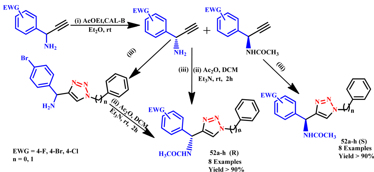
Scheme 41 Microwave-assisted synthesis of a-[4-(1-substituted)-1,2,3-triazol-4-yl]benzylacetamides. Conditions: (iii) (for n = 1 ) NaN 3 , benzyl chloride, sodium ascorbate/Cu(SO 4 ) 4 ·H 2 O/ t BuOH, MW, 125 °C, 10 min; (for n = 0 ) pHN 3 , sodium ascorbate/CuSO 4 ·H 2 O/ t BuOH, MW, 120 °C, 10 min. 82
