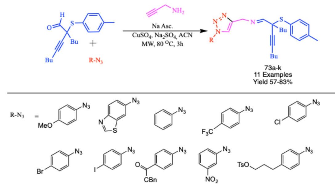
Scheme 62 Microwave-assisted synthesis of 1,2,3-triazoles (73a–k). 109
