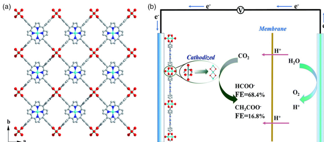
Fig. 14 (a) Crystal structure of \text{Cu}_2(\text{CuTCPP}) MOF nanosheets; (b) schematic of electrochemical system showing electrocatalytic reduction of \text{CO}_2 on \text{Cu}_2(\text{CuTCPP}) nanosheets. Reproduced with permission from Wu et al. 100 Copyright 2019, Royal Society of Chemistry.
