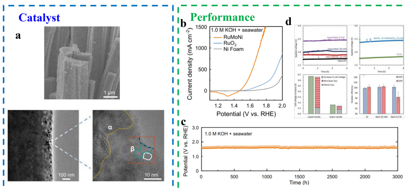
Fig. 6 (a) SEM and TEM images of the as-prepared RuMoNi electrocatalyst. 7 (b) Polarization curves of RuMoNi, RuO 2 , and Ni Foam in a 1.0 M KOH + seawater electrolyte at a scan rate of 5 \text{ mV s}^{-1} with 85% iR correction. 7 (c) Durability test for the OER for over 3000 h recorded at a current density of 500 \text{ mA cm}^{-2} in a 1.0 M KOH + seawater electrolyte. 7 (d) The electrochemical performance for the steam-fed anode and liquid-fed anode electrolysis cells. 35
