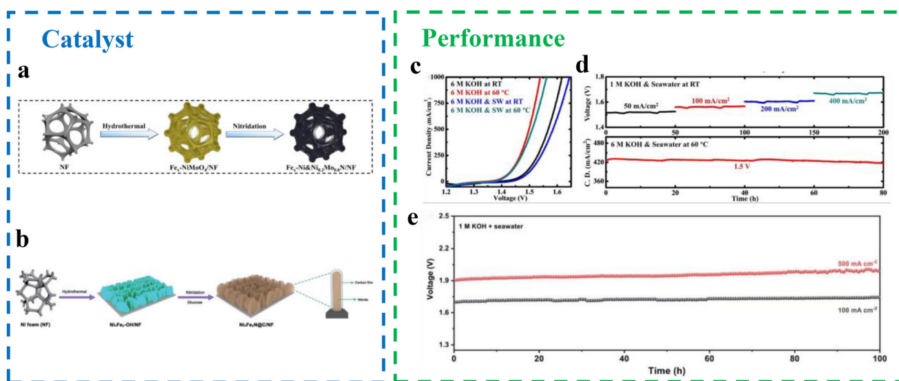
Fig. 19 (a) Synthesis process for Fe x -Ni&Ni 0.2 Mo 0.8 N microrods on NF. 83 (b) The preparation procedure of NiFeLDH@Ni 3 N/NF. 84 (c) Alkaline water and seawater electrolysis performance of Fe 0.01 -Ni&Ni 0.2 Mo 0.8 NFe 0.01 &Mo-NiO under industrial conditions. 83 (d) Stability measurements during alkaline seawater electrolysis. 83 (e) Durability tests of this electrolyzer at 100 and 500 mA cm -2 . 84
