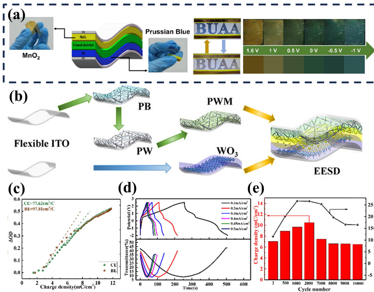
Fig. 6 (a) Schematic diagram of the flexible M-ECD and real photos (up) and emulsion images (down) at different voltages. Reproduced with permission. 133 Copyright 2023 American Chemical Society. Schematic illustration (b) and relevant characterizations (c–e) of the present EESD. Reproduced with permission. Copyright 2022 American Chemical Society.
