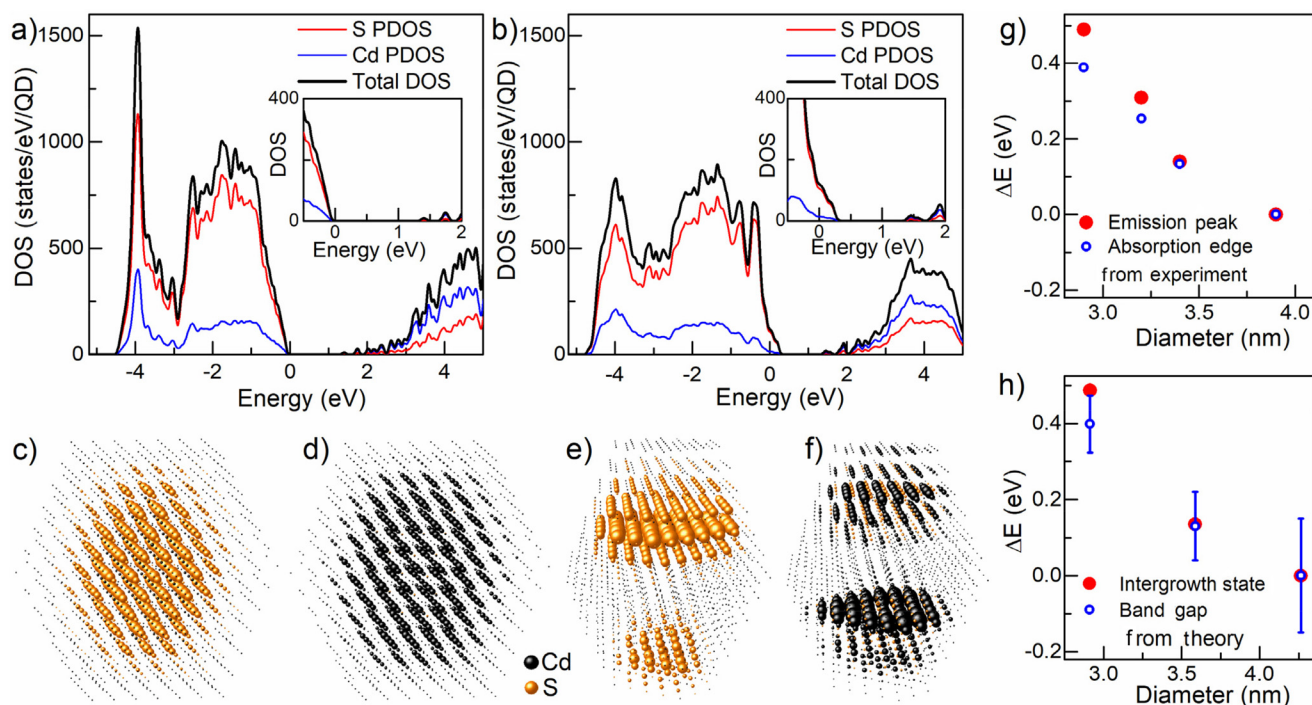
Fig. 4 Total and atom-resolved electronic density of states of (a) pristine ZnBr CdS QDs and (b) CdS QDs with the engineered interface of \sim 4 nm diameter. Insets in figures (a) and (b) show enlarged views of the band edge region. Weights of the wave functions of (c) the top of the occupied states (TOS) and (d) the bottom of the unoccupied states (BUS) of the same ZnBr CdS QD. Corresponding wave-function weights for (e) TOS and (f) BUS of the CdS QDs with an engineered interface of similar size. In (c)–(f), the size of the sphere at any atomic site is proportional to the total weight of the wave function at that site. Variation of intergrowth state energy and band gap with size (g) from experimental absorption and emission spectra and (h) from theoretically calculated electronic structure. These variations are shown with respect to the largest-sized QD considered in each case (experiment and theory).
