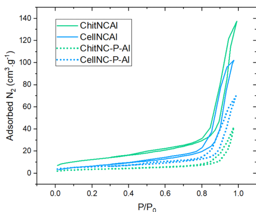
Fig. 9 N_2 adsorption–desorption isotherms (77 K) for spray-dried and calcined materials obtained with both polysaccharide nanocrystals (chitin and cellulose), phosphorylated or not, and reacted with Al_{13} clusters.
