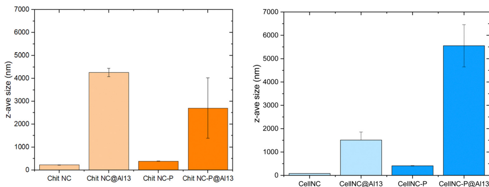
Fig. 6 Z-averaged hydrodynamic diameter measured by DLS for hybrid suspensions of (a) chitin and (b) cellulose nanocrystals after phosphorylation or not, in the presence or absence of \text{Al}_{13} clusters.
