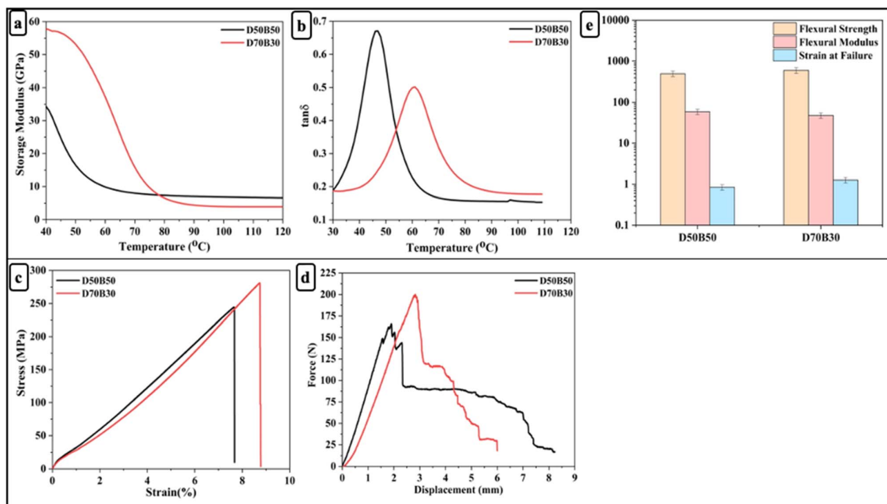
Fig. 5 (a) Storage modulus; (b) tan \delta ; (c) stress vs. strain curves; (d) force vs. displacement curves; (e) flexural strength, modulus, and strain at failure of D50B50 and D70B30 bio-based epoxy vitrimers.
