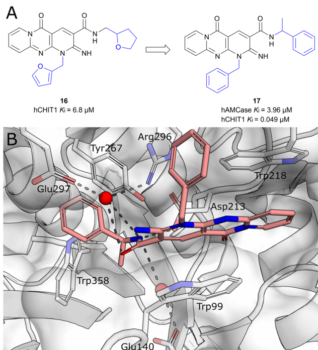
Fig. 10 A) Structure of dipyrrodo-pyrimidine analog 16 and optimization towards selective high-affinity CHIT1 inhibitor 17 . B) X-ray crystal structure of 17 in complex with CHIT1 (PDB ID 6JJR).
