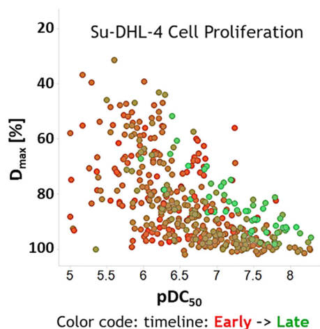
Fig. 3 Correlation between D_{\max} and pDC_{50} in Su-DHL-4 cell proliferation assay.
