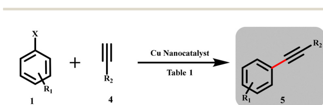
Scheme 2 Sonogashira cross-coupling reaction.
