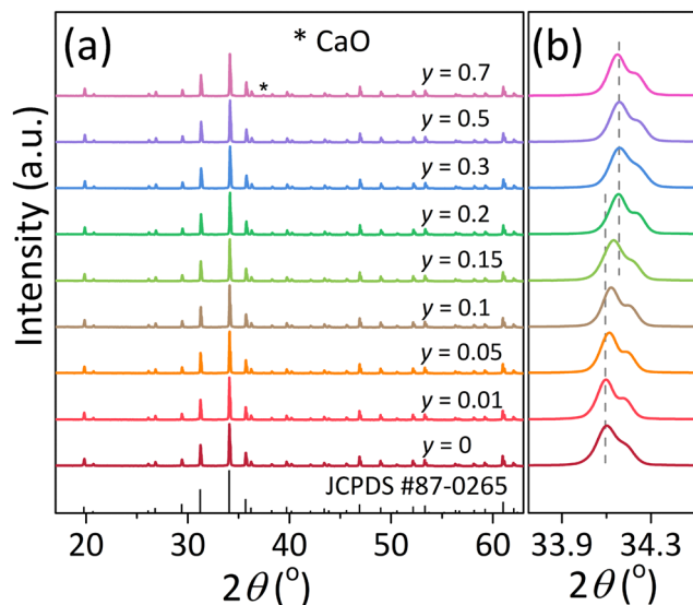
Fig. 3 (a) XRD patterns of the \text{Ca}_{14}\text{Zn}_6\text{Al}_{9.8-y}\text{B}_y\text{Mn}_{0.1}\text{Mg}_{0.1}\text{O}_{35} phosphors sintered at 1250\text{ }^\circ\text{C} for 5 h, (b) enlarged patterns around 2\theta = 34.1^\circ .
