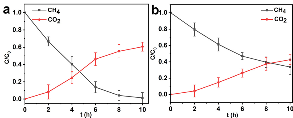
Fig. 9 Changes in \text{CH}_4 and \text{CO}_2 in the (a) HK@SB-T2 and (b) free cell methanotroph system (gas composition in the reactor was analyzed using gas chromatography every 2 hours). Error bars indicate the standard deviations of three independent experiments.
