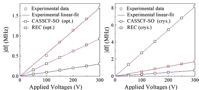
Fig. 2 The shift in transition frequency ( \delta f ) versus applied voltage V , showing a linear E-field coupling in HoW 10 . Calculations correspond to the DFT-optimized structure (left) and to the crystallographic structure (right). 51
