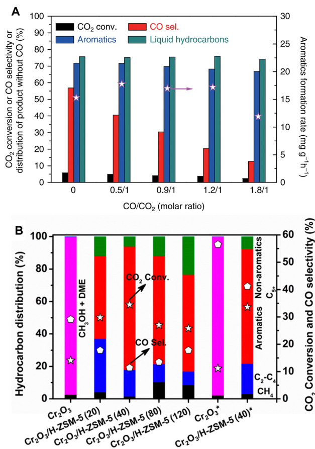
Fig. 17 The coupling of CO 2 hydrogenation with CO hydrogenation. (A) 667 mg of ZnAlO 3 /H-ZSM-5, 320 °C, 3.0 MPa, H 2 /CO 2 /Ar = 3/1/0.2, 66.7 mL min -1 , CO = 0–26.6 mL min -1 . Reprinted with permission from Ni et al. Copyright (2018), The Authors. 41 (B) 0.25 g of Cr 2 O 3 /H-ZSM-5, 350 °C, 3 MPa, H 2 /CO 2 = 3 (5.42 vol% CO), 10 mL min -1 . * refers to the results without CO. Reprinted with permission from Wang et al. Copyright (2019), American Chemical Society. 55
