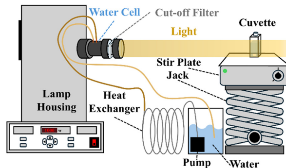
Scheme 1 Photochemical setup with a 1.0 kW Xe (Hg) lamp filtered through water to remove infrared radiation, and equipped with a cut-off filter at \lambda_{\text{cut-off}} \geq 295 \text{ nm} .
