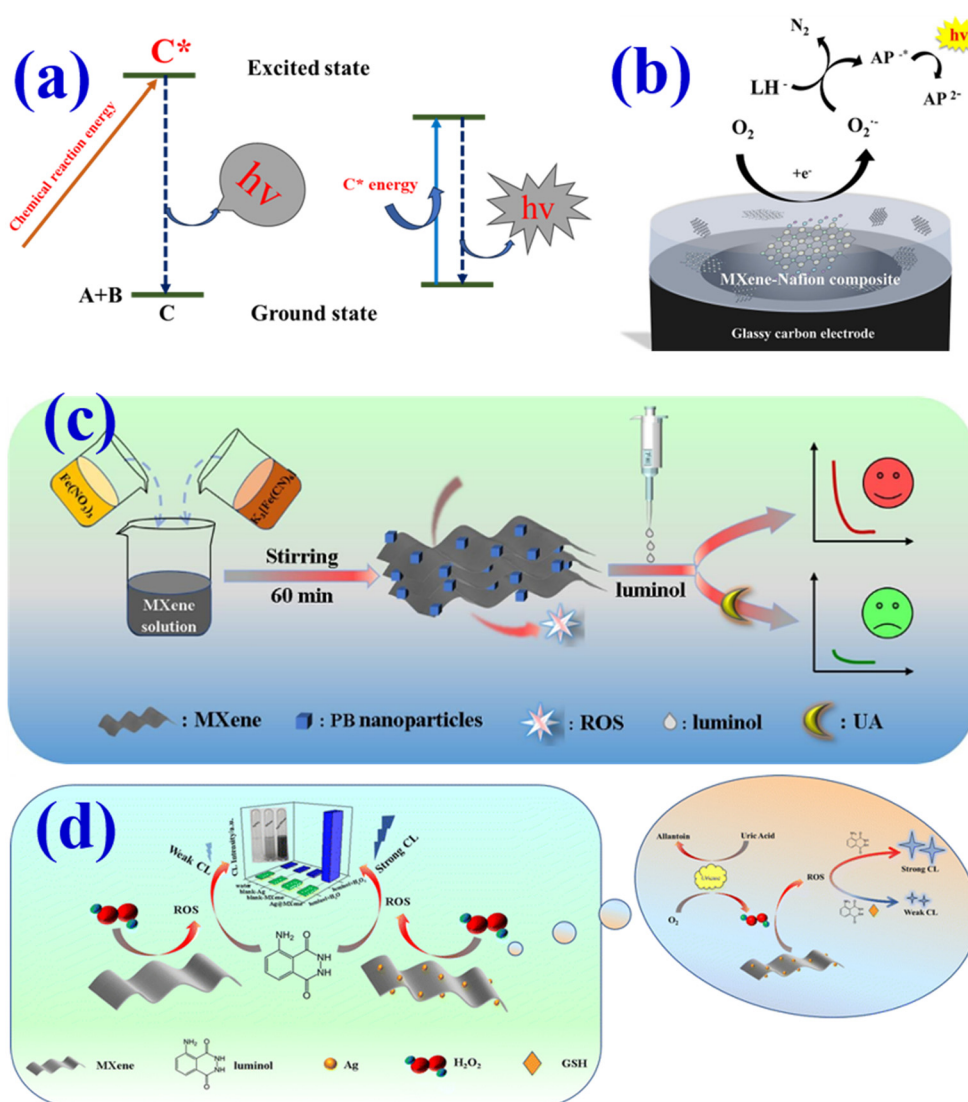
Fig. 9 (a) Schematic illustration of the formation of the CL mechanism. MXzyme-based CL sensors for important analytes. (b) Glassy carbon (GC) electrode modified with a 2D \text{Ti}_3\text{C}_2\text{T}_x MXene–Nafion composite material [reproduced from ref. 207 with permission from Elsevier, copyright 2023], (c) PB/ \text{Ti}_3\text{C}_2\text{T}_x MXene nanocomposite-based CL detection of UA [reproduced from ref. 208 with permission from Elsevier, copyright 2024], and (d) Ag/MXene nanozymes for efficient CL sensing of UA and GSH [reproduced from ref. 211 with permission from Royal Society of Chemistry, copyright 2024].
