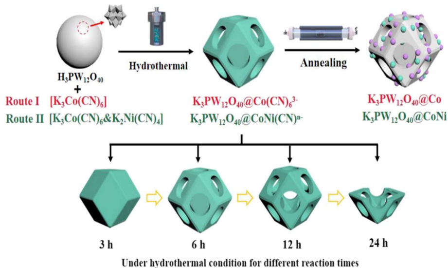
Fig. 3 Schematic illustration of the formation of the hydrothermal intermediate product \text{K}_3\text{PW}_{12}@\text{Co}(\text{CN})_6^{3-}/\text{K}_3\text{PW}_{12}@\text{CoNi}(\text{CN})^n and the annealed product \text{K}_3\text{PW}_{12}@\text{Co}/\text{K}_3\text{PW}_{12}@\text{CoNi} . 85
