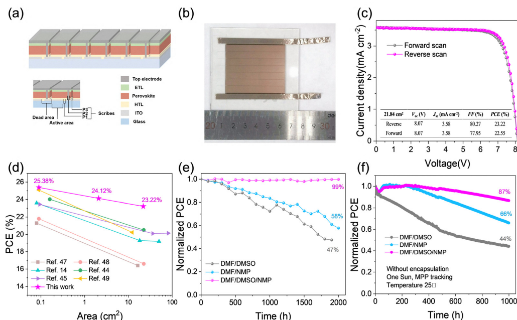
Fig. 5 (a) Schematic diagram of the perovskite mini-module. (b) Digital photograph and (c) J - V curves of the best-performing mini-module on a 7.6 \text{ cm} \times 7.6 \text{ cm} substrate based on the DMF/DMSO/NMP solvent system. (d) Comparison of the efficiency decline during upscaling of the present work with those previously reported in the literature. 14,44,45,47–49 (e) Evolution of PCE of the unencapsulated blade-coated PSCs in an \text{N}_2 -filled glove box. (f) MPP tracking of PSCs under one sun illumination.
