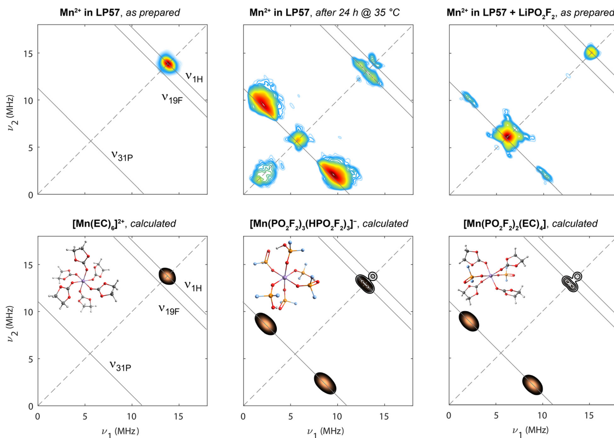
Fig. 2 Experimental (upper row) and calculated (lower row) HYSCORE spectra at 9.8 GHz (X-band; 20 K). Spectra from samples containing 8 mM \text{Mn(TFSI)}_2 dissolved in 1 M \text{LiPF}_6 in 3:7 EC:EMC (left), with mild heat-treatment at 35 °C for 24 h (centre), and addition of 80 mM \text{LiPO}_2\text{F}_2 (right) are shown. Experiments were conducted at the magnetic field positions indicated by green arrows in Fig. 1. The diagonal is shown with a dashed line. Anti-diagonal (solid) lines are shown at relevant nuclear Larmor frequencies. Calculations are shown for three clusters, [\text{Mn}(\text{EC})_6]^{2+} , [\text{Mn}(\text{PO}_2\text{F}_2)_3(\text{HPO}_2\text{F}_2)_3]^- and [\text{Mn}(\text{PO}_2\text{F}_2)_2(\text{EC})_4] .
