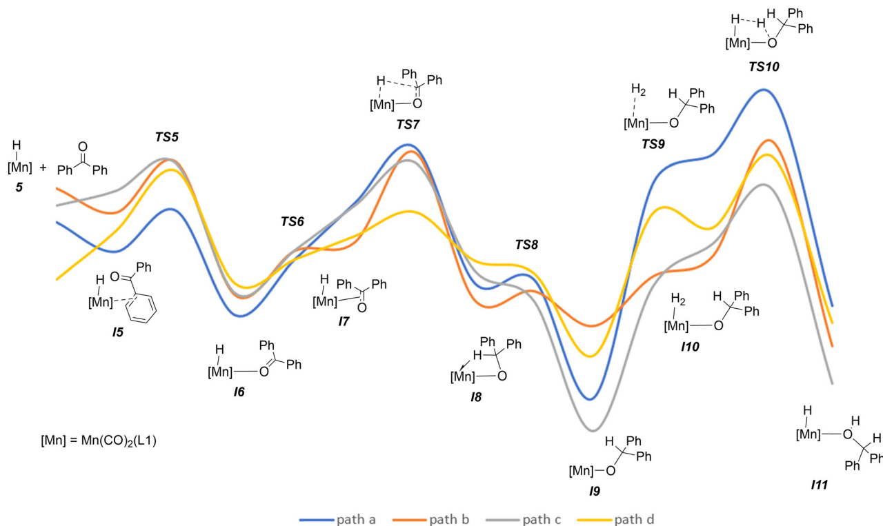
Fig. 12 Free energy profiles for benzophenone hydrogenation catalysed by Mn(H)(L1)(CO) 2 .
