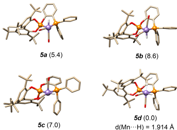
Fig. 11 Optimized geometries for Mn(H)(L1)(CO) 2 isomers ( 5a–5d ). Numerical values correspond to relative free energies in kcal mol -1 relative to 5d . Hydrogens have been omitted for clarity except those of the methyl involved in an agostic interaction in 5d .
