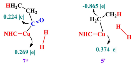
Fig. 6 The NBO charges on the Cu atom and C atom in intermediate 7* and intermediate 5'. The values have been indicated in green.
