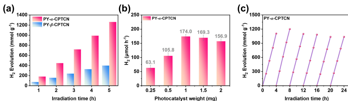
Fig. 2 (a) Hydrogen evolution versus time of PY- \alpha -CPTCN and PY- \beta -CPTCN NPs at the concentration of 5 \mu\text{g mL}^{-1} , under AM 1.5G ( 100 \text{ mW cm}^{-2} ). (b) Photocatalytic \text{H}_2 evolution patterns of PY- \alpha -CPTCN NPs with different weights of the photocatalyst. (c) Time course hydrogen evolution curve of PY- \alpha -CPTCN NPs.
