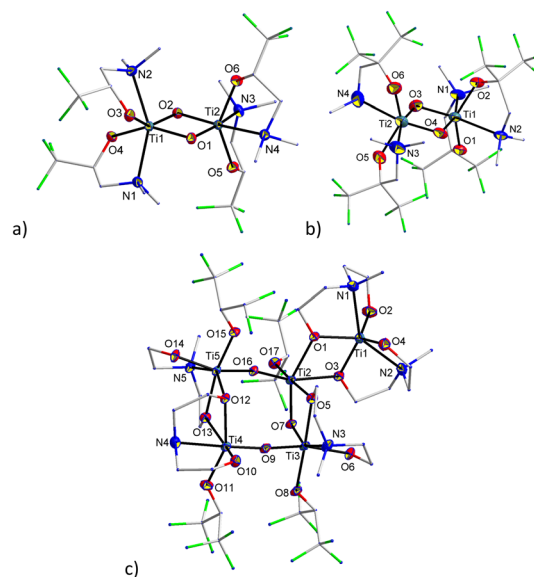
Fig. 2 Molecular structures of (a) [\text{Ti}_2(\mu\text{-O})_2(\eta^2\text{-F-dmap})_4] ( 9 ), (b) [\text{Ti}_2(\mu\text{-O})_2(\eta^2\text{-F-dmamp})_4] ( 10 ) and (c) [\text{Ti}_5(\mu\text{-O})_3(\mu\text{-mdea})_5(\eta^1\text{-hfip})_4] ( 11 ) with displacement ellipsoids drawn at the 50% probability level. H atoms are omitted for clarity.
