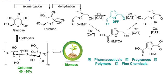
Scheme 1 Furan-based platform molecules with plausible reaction pathways from cellulose.
