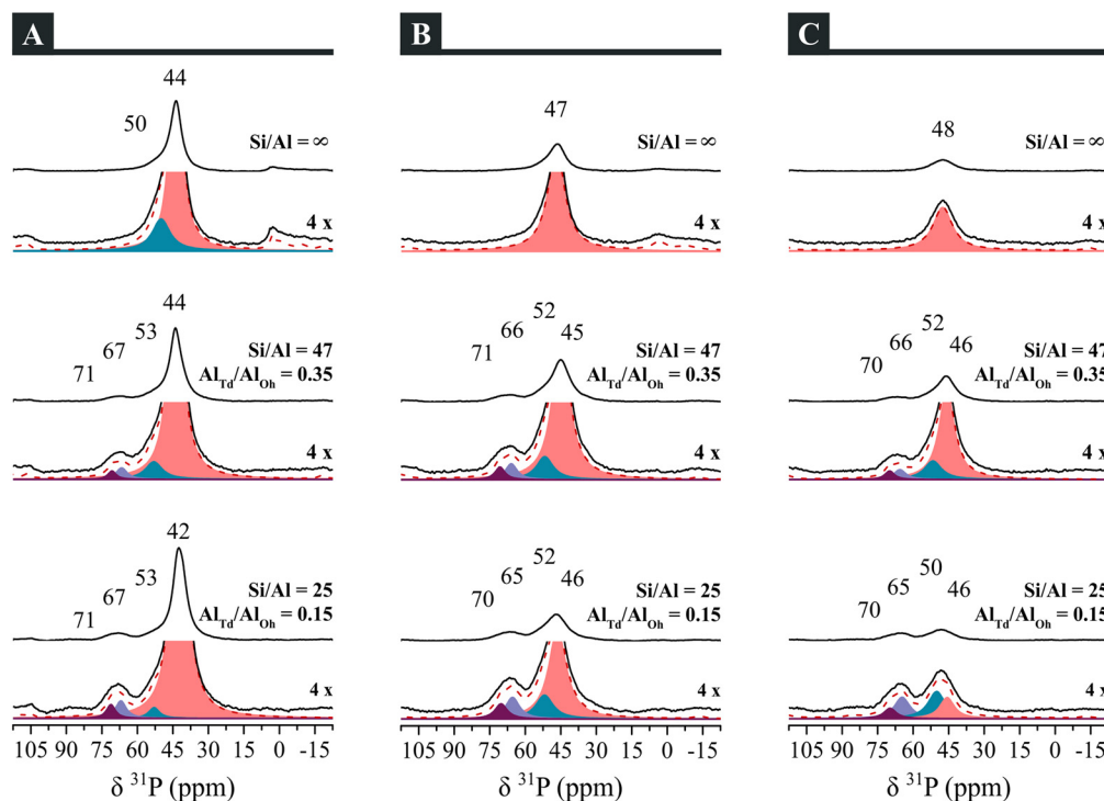
Fig. 4 31 P-MAS-NMR spectra for H-R18 and H-[Al]-R18 seeded samples in the absence of water, with different Si/Al and Al Td /Al Oh molar ratios and P/Al molar ratios = (A) 1.4, (B) 0.50, and (C) 0.25. The deconvoluted signals were magnified 4×.
