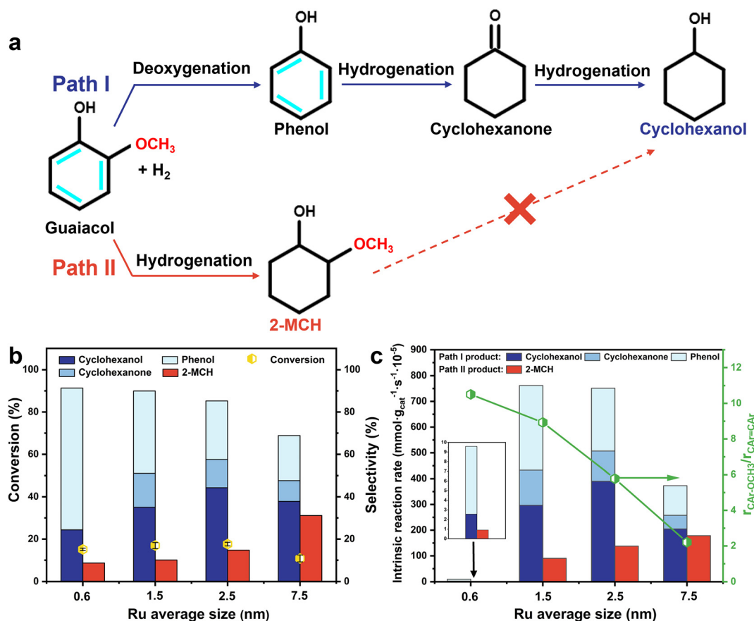
Fig. 4 a. Two estimated reaction pathways (guaiacol → phenol → cyclohexanone → cyclohexanol and guaiacol → 2-MCH) of HDO of guaiacol on the Ru/γ-Al 2 O 3 catalysts; b. selectivity toward major products on catalysts with different Ru average sizes at ~15% guaiacol conversion (reaction conditions: 190 °C, 5 bar H 2 , 3.0 mL H 2 O, 0.3 mmol guaiacol, the error bars show the deviation of guaiacol conversion based on three repeated experiments); c. mass-specific intrinsic reaction rate of different products on Ru/γ-Al 2 O 3 catalysts with different Ru particles and relative ratio of the C Ar -OCH 3 bond cleavage rate ( r_{C_{Ar}-OCH_3} ) and aromatic ring hydrogenation rate ( r_{C_{Ar}=C_{Ar}} ) of guaiacol (reaction conditions of Ru 0.6 /γ-Al 2 O 3 : 0.3 mmol guaiacol, 0.02 g catalyst, 3.0 mL H 2 O, 5 bar H 2 , 190 °C, 6 h, 400 rpm; reaction conditions of Ru 1.5 /γ-Al 2 O 3 , Ru 2.5 /γ-Al 2 O 3 and Ru 7.5 /γ-Al 2 O 3 : 0.3 mmol guaiacol, 0.01 g catalyst, 3.0 mL H 2 O, 5 bar H 2 , 190 °C, 1/6 h, 400 rpm).
