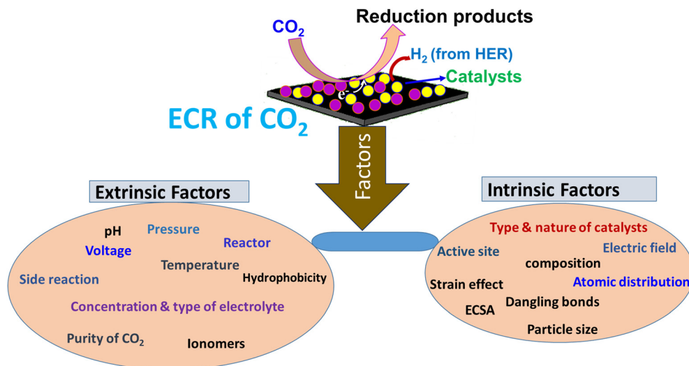
Fig. 6 Extrinsic and intrinsic factors affecting the ECR of CO 2 .
