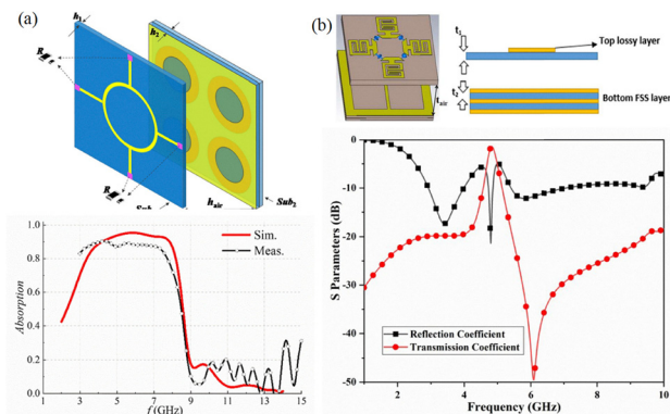
Fig. 19 (a) Tunable frequency-selective rasorber. Reproduced from ref. 158 with permission from Radio Science, copyright 2021. (b) Novel compact open-loop resonator-loaded rasorber. Reproduced from ref. 159 with permission from Progress In Electromagnetics Research M, copyright 2025.
