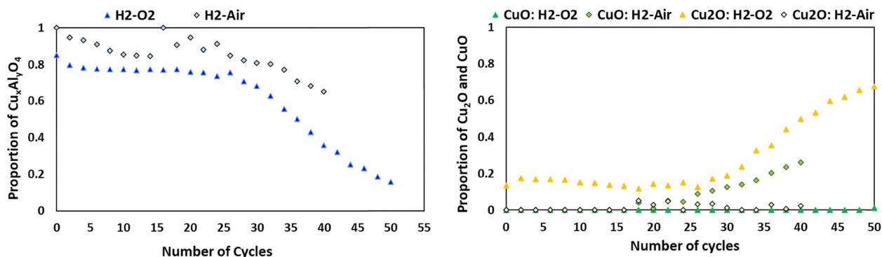
Fig. 6 Changes in the relative percentages of \text{Cu}_x\text{Al}_y\text{O}_4 (left) and \text{Cu}_2\text{O}-\text{CuO} phases (right) at the end of the oxidation reactions from fresh sample to up to 50 cycles for \text{H}_2-\text{O}_2 and \text{H}_2 -air datasets.
