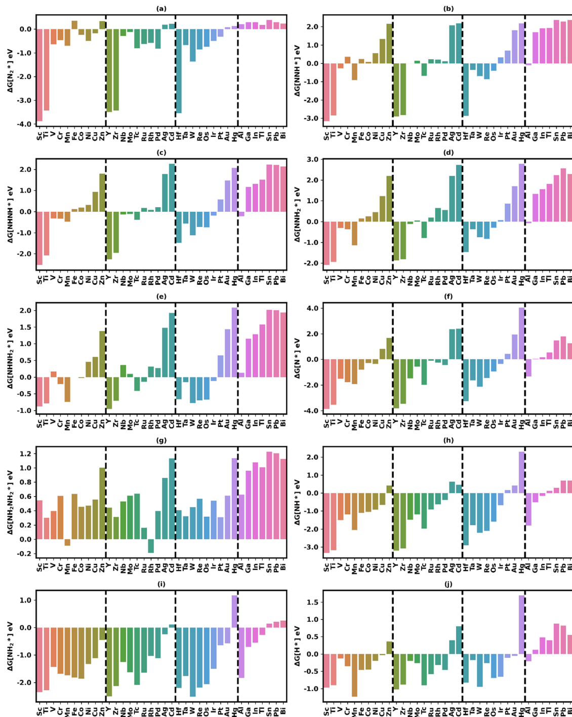
Fig. 2 Adsorption free energies ( \Delta G ; eV) of key NRR intermediates, including (a) N_2^* , (b) NNH^* , (c) NHNH^* , (d) NNH_2^* , (e) NHNH_2^* , (f) N^* , (g) NH_2NH_2^* , (h) NH^* , (i) NH_2^* and (j) H^* on various metal nanoclusters. The panels highlight distinct trends in adsorption free energies across early, mid, and late transition metals, as well as p-block and pseudo-p block metals.
