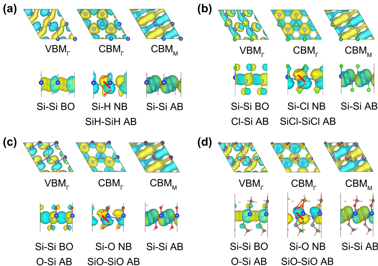
Fig. 3 The top and side views of the VBM _{\Gamma} , CBM _{\Gamma} , and CBM _M orbitals of (a) SiH, (b) SiCl, (c) SiOH, and (d) SiOCH 3 . The characters of the orbitals with respect to certain pairs of atoms are specified: BO = bonding orbital, NB = nonbonding, and AB = antibonding.
