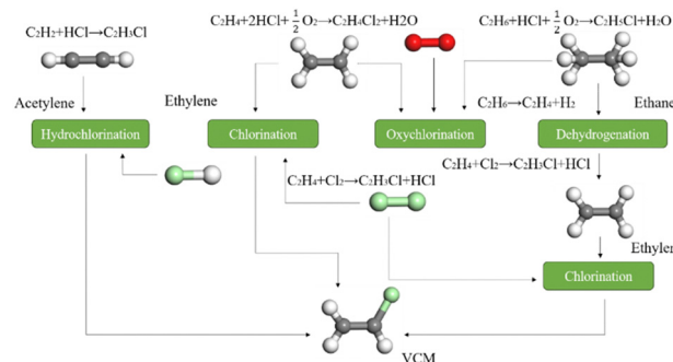
Fig. 1 Schematic illustration of various PVC synthesis routes.
