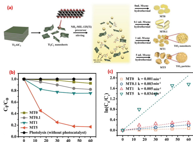
Fig. 15 (a) Synthesis scheme of Ti 3 C 2 /MOF heterostructures; (b) photocatalytic degradation of TC-HCl ( \lambda > 420 nm) of all as-synthesized samples; and (c) pseudo first-order kinetic fitting curves. Reprinted with permission from ref. 39. Copyright 2020 Elsevier.
