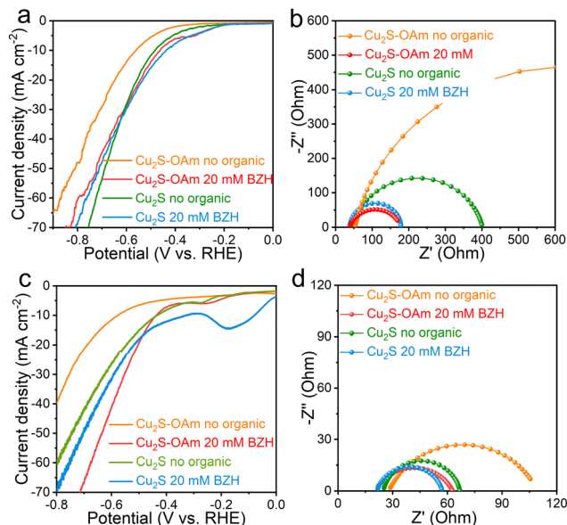
Fig. 3 (a) LSV curves and (b) Nyquist plots at -0.7 V vs. RHE of Cu 2 S-OAm and Cu 2 S in 1 M sodium acetate-acetic acid electrolyte (pH = 5.2) with and without BZH at room temperature; (c) LSV curves and (d) Nyquist plot at -0.7 V vs. RHE of Cu 2 S-OAm and Cu 2 S in 1 M potassium carbonate-potassium bicarbonate electrolyte (pH = 9) with or without BZH at room temperature.
