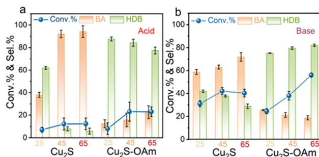
Fig. 5 BZH conversion and selectivity toward BA and HDB after 20 min reaction on \text{Cu}_2\text{S} and \text{Cu}_2\text{S} -OAm electrodes at -0.8 V vs. RHE, 25 ^{\circ}\text{C} , 45 ^{\circ}\text{C} or 65 ^{\circ}\text{C} in (a) 1 M sodium acetate-acetic acid solution ( \text{pH} = 5.2 ) with 20 mM BZH; (b) 1 M potassium carbonate-potassium bicarbonate solution ( \text{pH} = 9.0 ) with 20 mM BZH.
