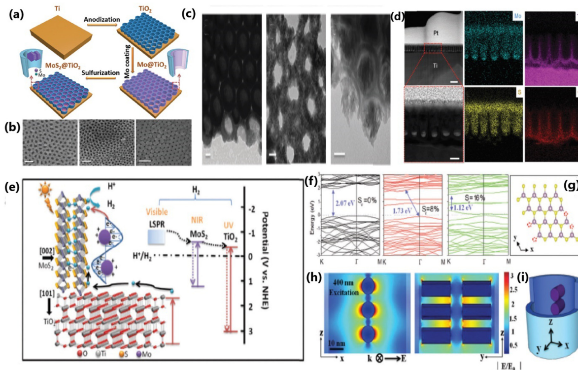
Fig. 10 (a) Schematic illustration of the assembly process of the MoS 2 @TiO 2 heterostructure. (b) SEM pictures of MoS 2 (10)@TiO 2 , MoS 2 (20)@TiO 2 and MoS 2 (30)@TiO 2 , respectively (scale bar: 100 nm). (c) TEM and HRTEM images of MoS 2 (10)@TiO 2 and MoS 2 (20)@TiO 2 (scale bar: 20 nm). (d) Cross-sectional HAADF-STEM images and EDS elemental mapping of the MoS 2 @TiO 2 heterostructure (first row, scale bar: 200 nm, and second row, scale bar: 50 nm). (e) Schematic diagram of the energy band structure, plasmonic resonance and electron transfer pathway in the MoS 2 @TiO 2 heterojunction. (f) Band structure of monolayer 2H-MoS 2 with 0%, 8% and 16% S-vacancies, with the valence band maximum and conduction band minimum both at the K point. (g) Model used for band gap computation via DFT. (h) FEM simulation of the near-field electric field distribution inside MoS 2 @TiO 2 heterostructures excited by a 400 nm laser and (i) 3D-simplified model used for FEM simulation. Reproduced with permission from ref. 139. Copyright ©2018, The Royal Society of Chemistry.
