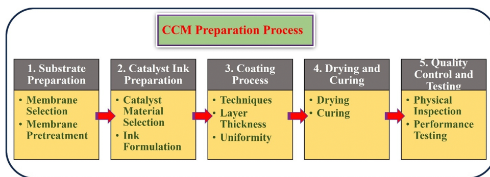
Fig. 3 Schematic sketch of the CCM preparation process.
