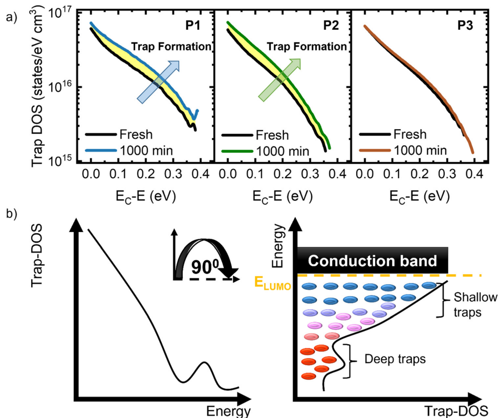
Fig. 5 (a) Trap DOS spectra before and after bias stress in OFETs based on each of the three polymers. (b) (Left) Distribution of traps within the polymer bandgap: shallow traps are located near band edges (tail states) and deep traps form a distinct peak. (Right) Schematic representation of the spatial and energy diagram of trap-DOS consisting of acceptor-like shallow and deep traps.
