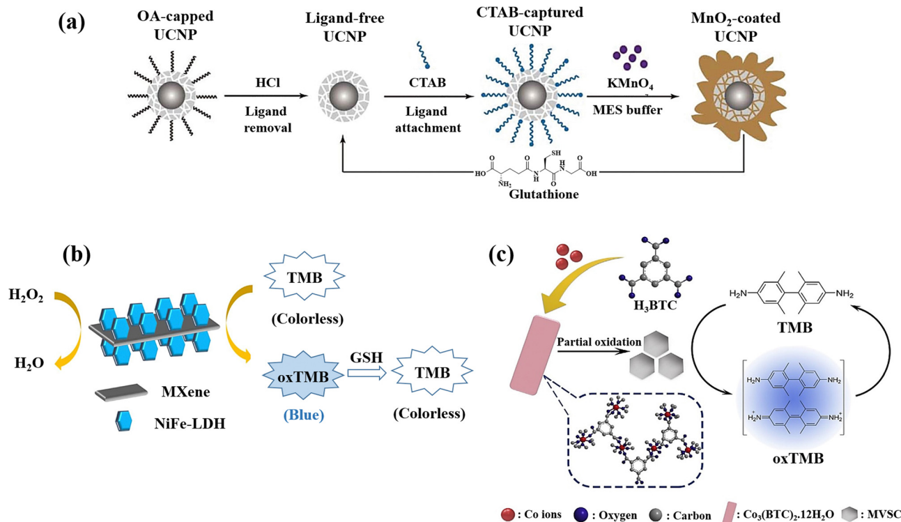
Fig. 11 (a) Graphical representation of surface alteration and GSH recognition by employing the \alpha - \text{NaYbF}_4 :Tm (1%)@ \text{CaF}_2 core-satellite UCNP. 22 (b) Colourimetric GSH detection via MXene@NiFe-LDH nanocatalyst. 76 (c) Diagram of preparation of \text{Co}_3(\text{BTC})_2 \cdot 12\text{H}_2\text{O} and mixed-valence-state cobalt (MVSC), as well as colourimetric sensor for GSH detection 77 reproduced with the permission of Royal Society of Chemistry, American Chemical Society, and Elsevier.
