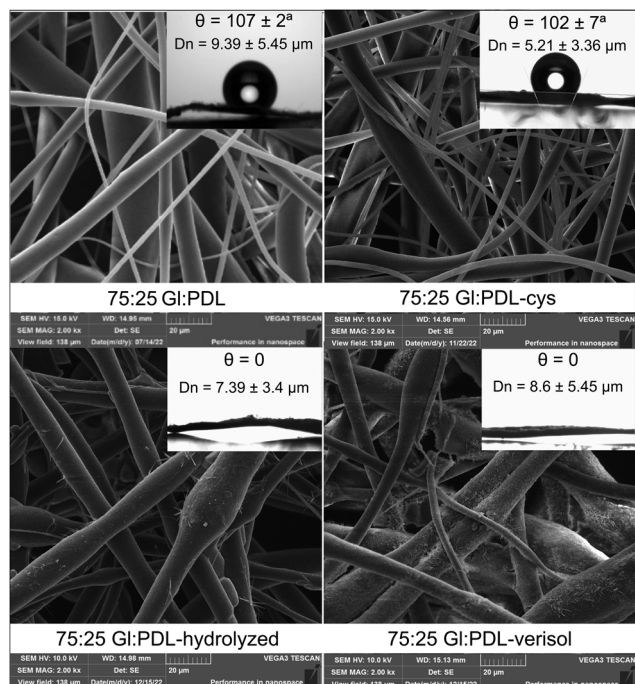
Fig. 3 Morphology, number average fiber diameter ( D_n ) and water contact angles ( \theta ) of 75:25 Gl:PDL raw scaffolds after functionalization with cysteine (75:25 Gl:PDL-cys) and after bioconjugation with hydrolyzed and with Verisol ® collagens, respectively, (75:25 Gl:PDL-hydrolyzed) and (75:25 Gl:PDL-verisol).
